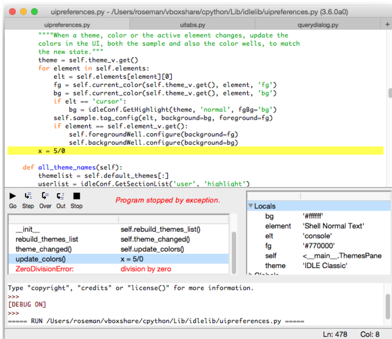
Early mockup of window integration (macOS).
