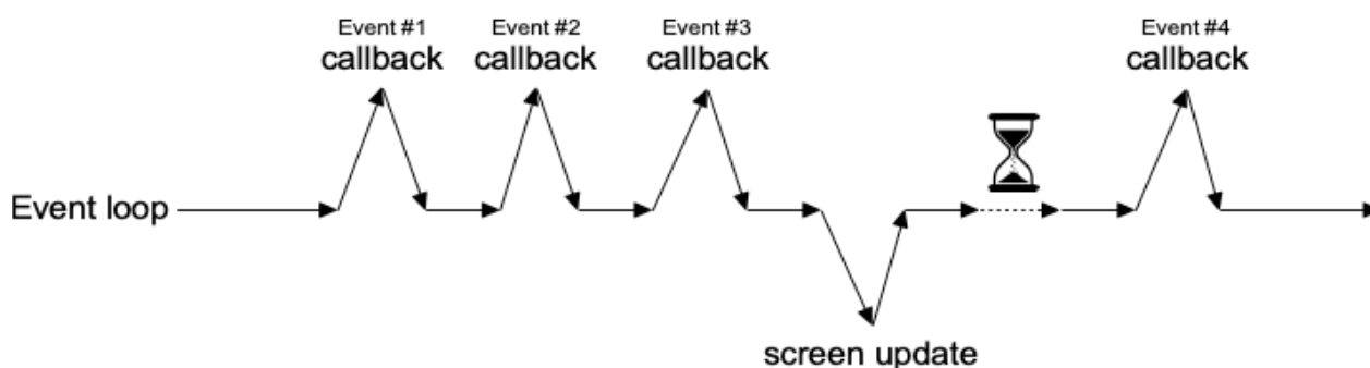
Execution timeline for a well-behaved event loop.
