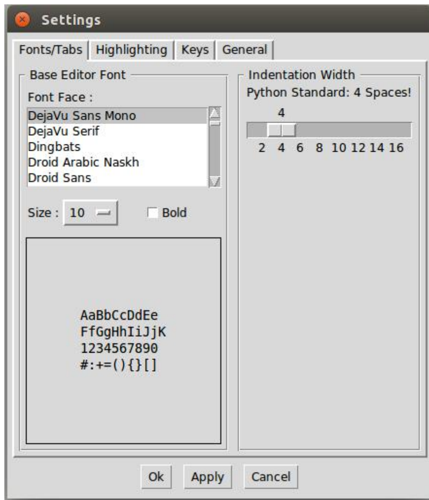
IDLE's Preferences window (Linux).
