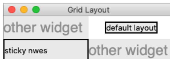
Layout within the cell and the 'sticky' option.
