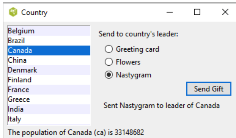
Country selector listbox example.
