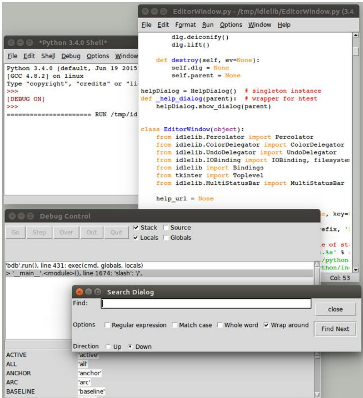
Overview of IDLE user interface (on Linux).
