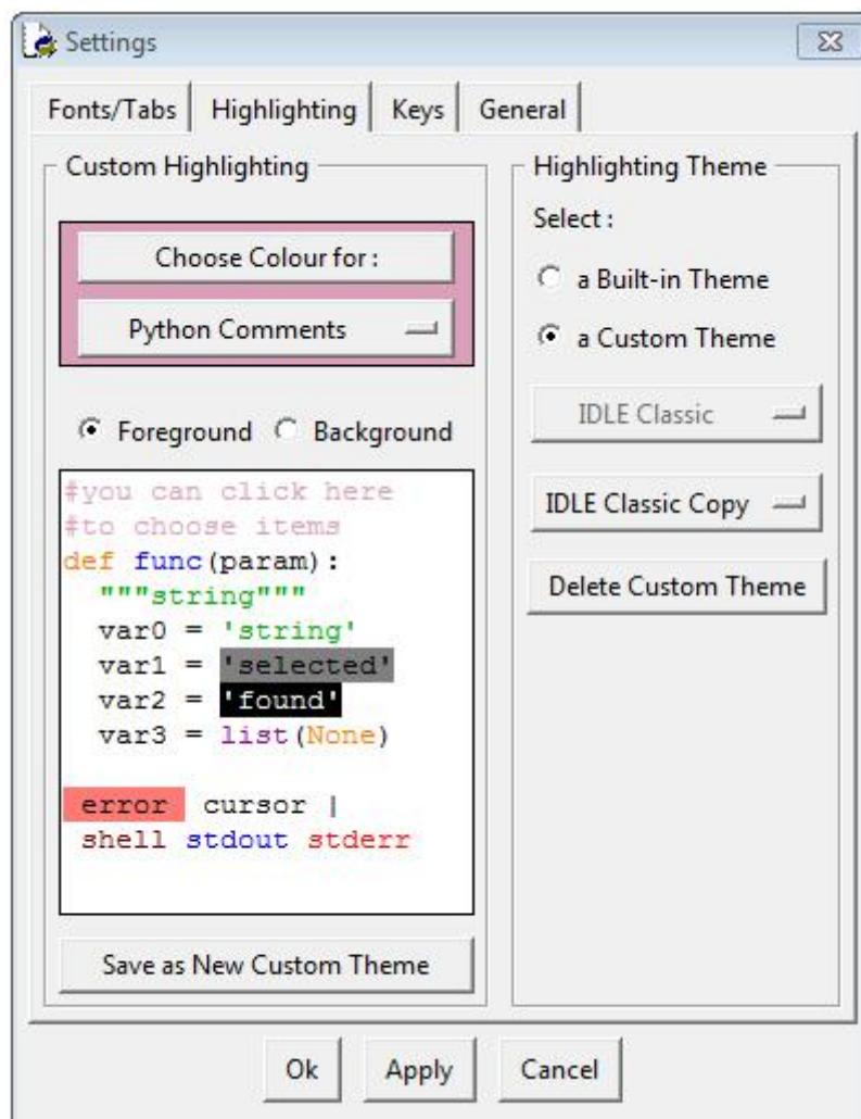
IDLE Themes pane, before (Windows).
