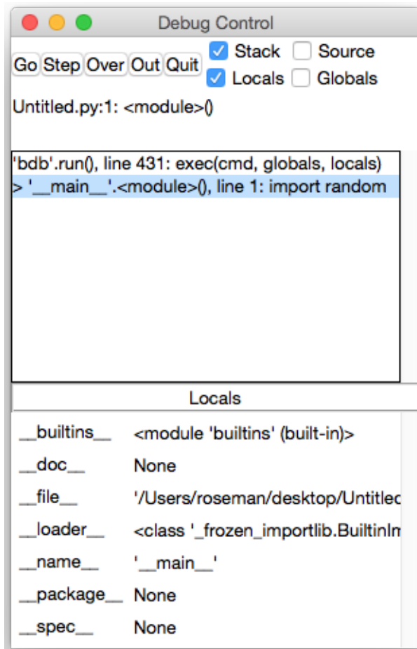
Original IDLE debugger (macOS).
