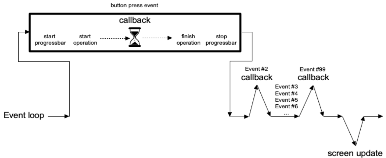
Lengthy callback blocking the event loop.
