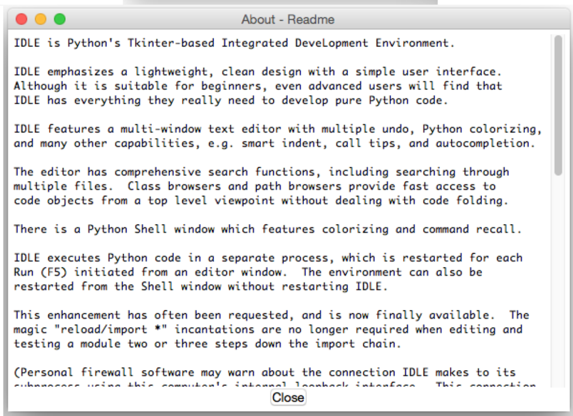
IDLE's doubly-modal About dialog (macOS).
